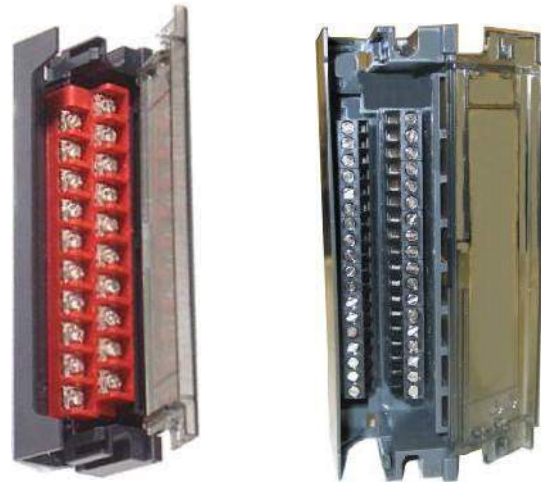
Sample terminal blocks (L) 20-terminal high voltage Barrier (R) 36-terminal Euro
