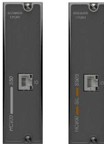
Process Scanner (left) Safety Scanner (right)
