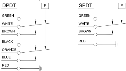
WIRING DIAGRAM FOR CABLE
