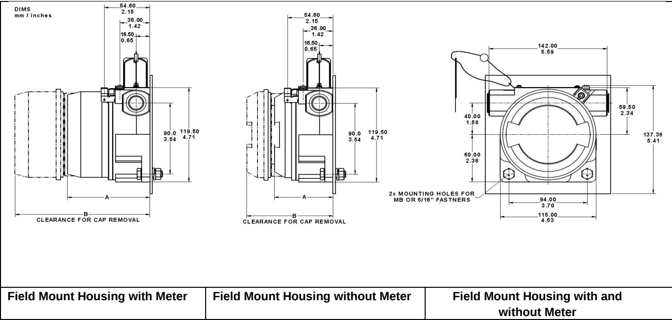
Figure 4: Wall Mounting Dimensions
