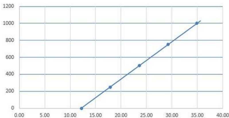
STT700 Load Line - HART
