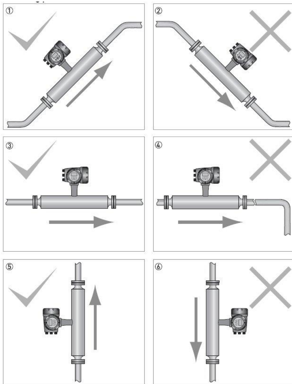
Figure 12 – Mounting Position
