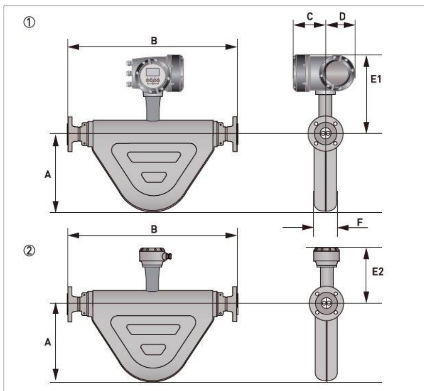
Figure 7 – Meter Dimensions
